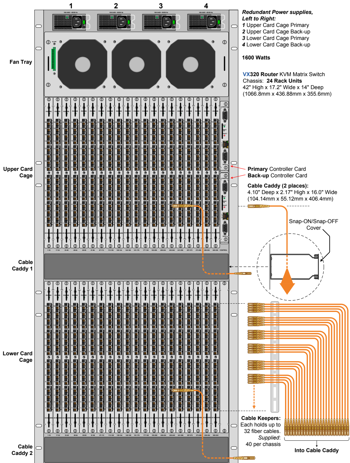
Figure 1a. Thinklogical VX 320 Router
