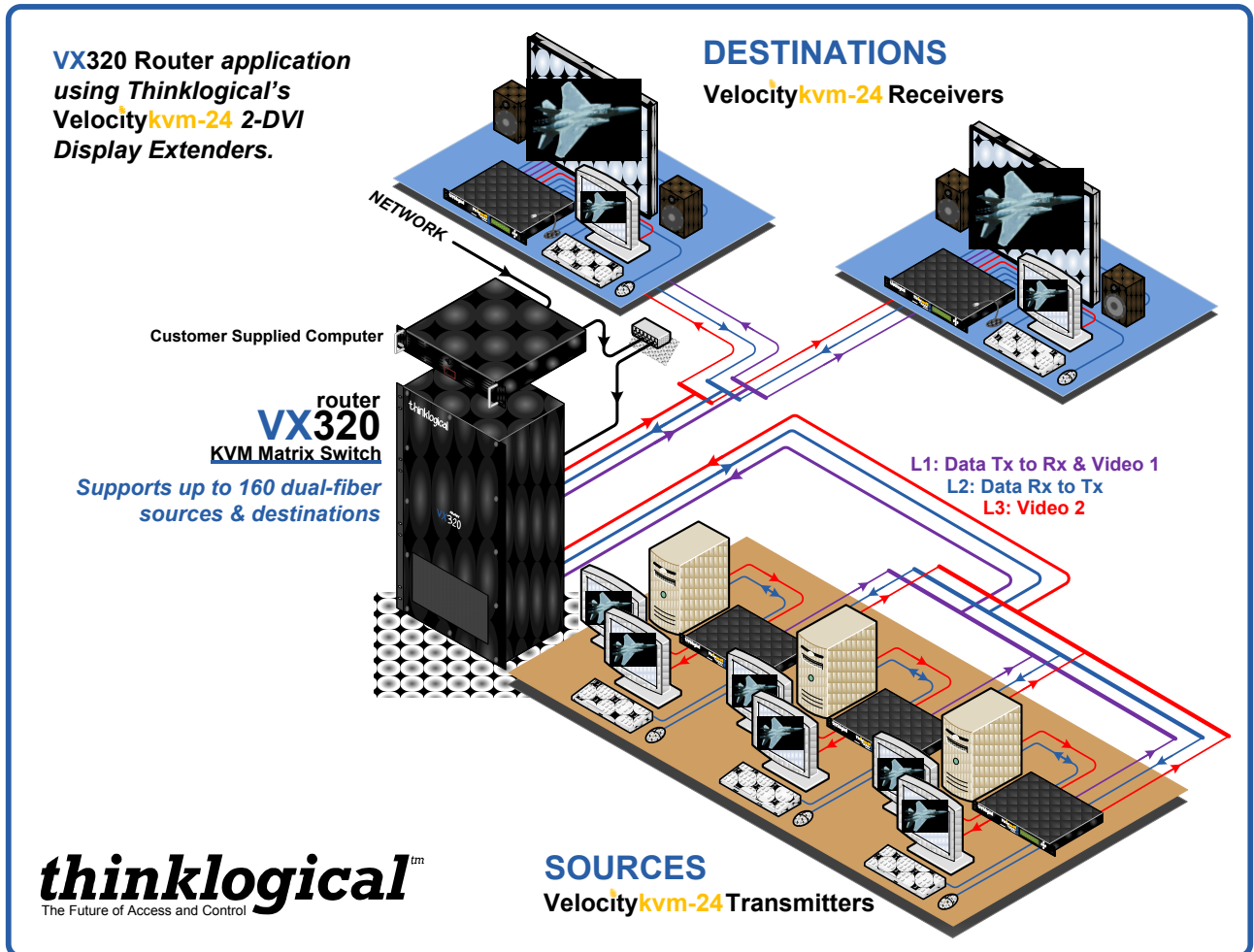
Figure 2a. Typical TOE VX320 Configuration
